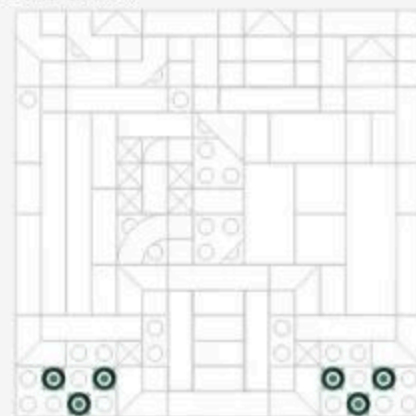
Vertical View of Installation Drawing 安装图顶面
