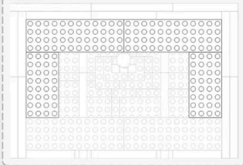
Vertical View of Installation Drawing 安装图顶面
