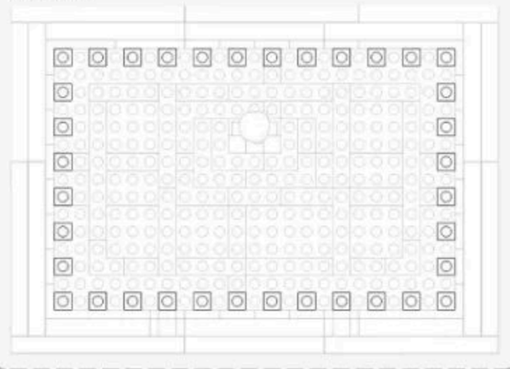
Vertical View of Installation Drawing 安装图顶面
