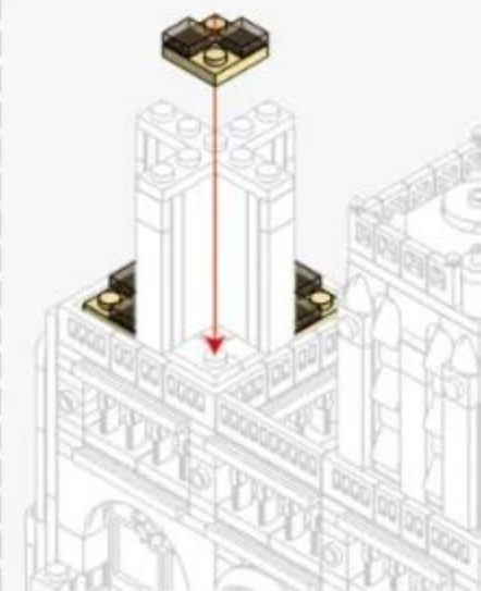
Back Side of Installation Drawing 安装图背面
