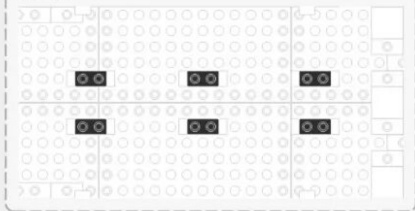
Vertical View of Installation Drawing 安装图顶面
