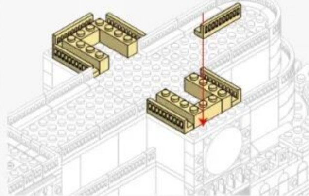
Back Side of Installation Drawing
