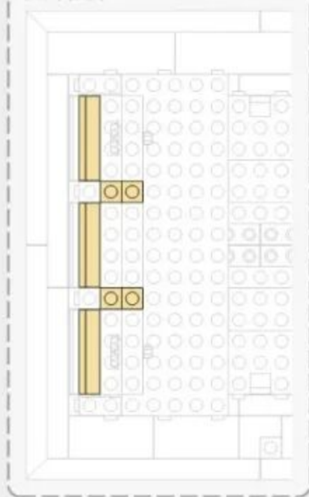
Vertical View of Installation Drawing 安装图顶面
