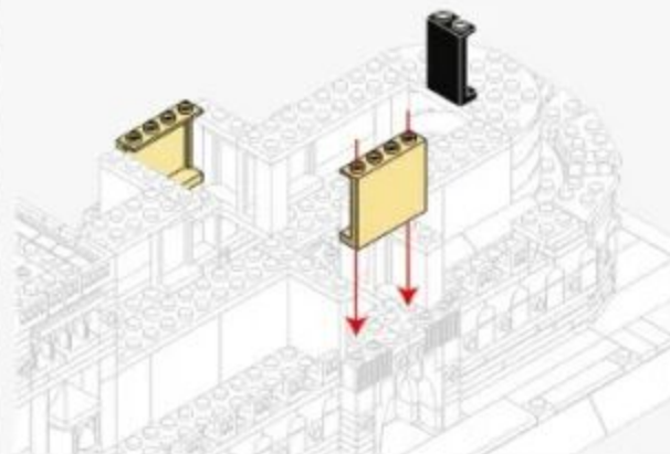
Back Side of Installation Drawing 安装图背面
