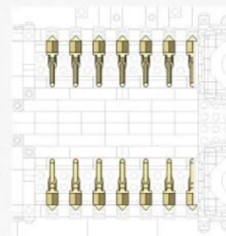
Vertical View of Installation Drawing 安装图顶面
