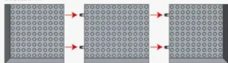
Vertical View of Installation Drawing 安装图顶面
