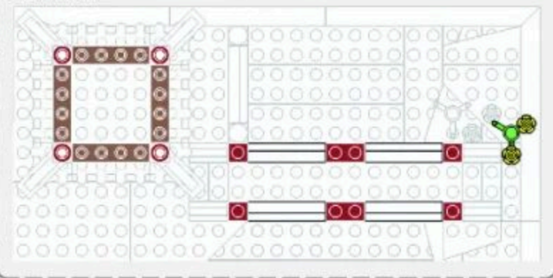
Vertical View of Installation Drawing 安装图顶面
